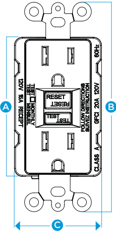
FRONT DIMENSIONS
